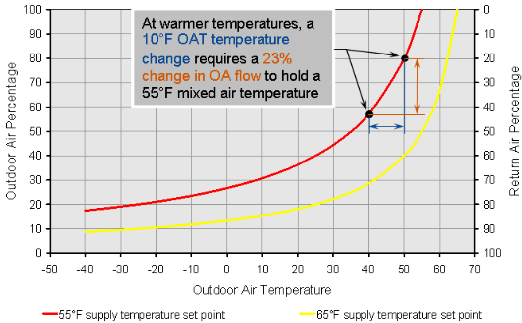
Figure 12 – Economizer non-linearity
