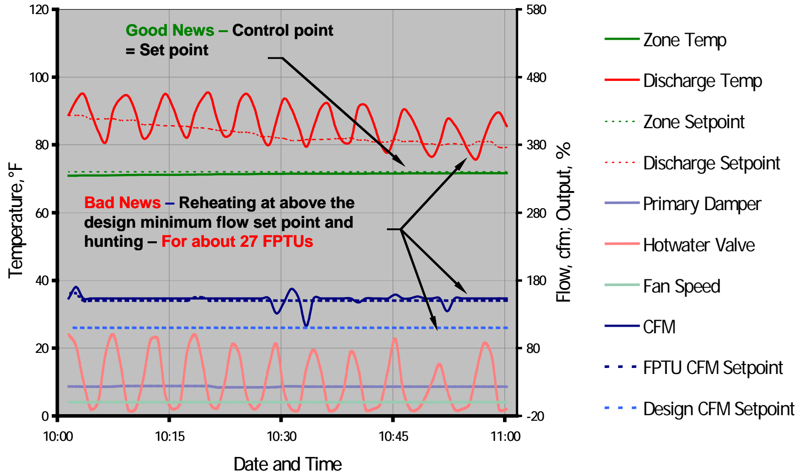
Figure 3 – Thermal inertia and a reheat process mask instability and excess ventilation in a fan-terminal unit.
