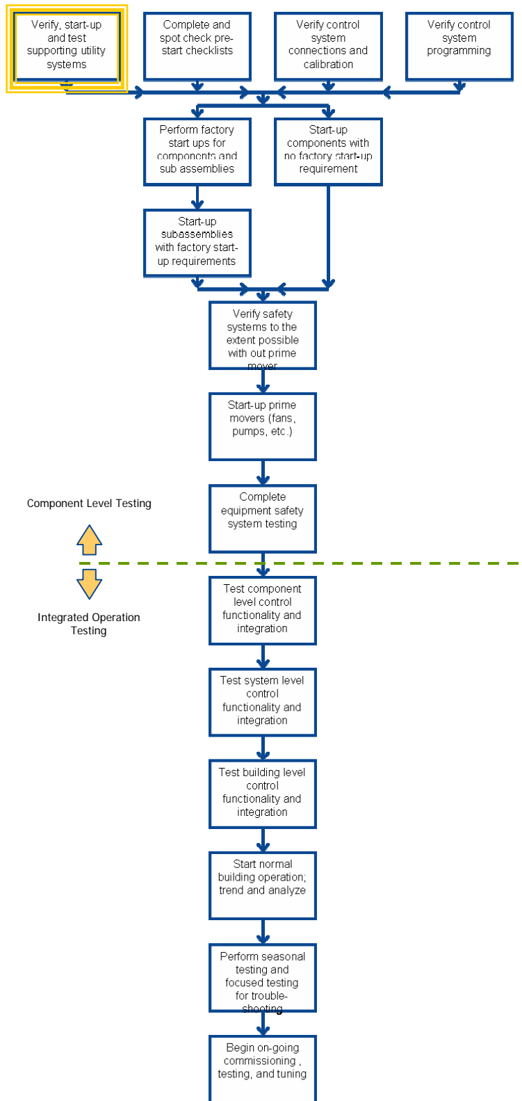
Figure 4 – A typical testing hierarchy. The functions in the box highlighted in gold could have this entire testing hierarchy associated with it.
