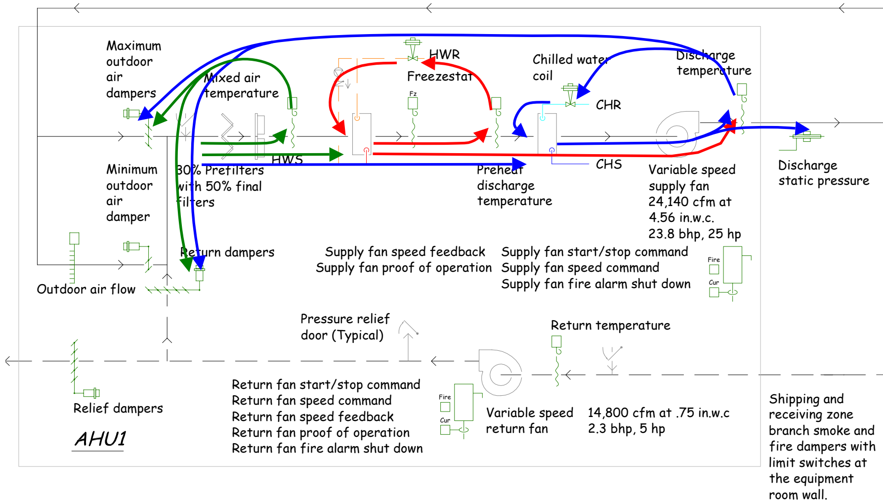
Figure 1 –AHU1 temperature-control processes interaction potential. The blue lines represent the discharge-temperature control loop and the impact of the cooling coil and economizer dampers that it controls. The green lines represent the mixed-air- low-limit temperature control loop and the impact of the economizer dampers it limits. The red lines represent the preheat discharge temperature control loop and the impact of the preheat coil it controls.
